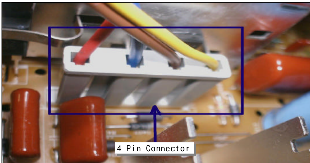
AFTER : CDT DY CONNECTOR (4 pin type)
